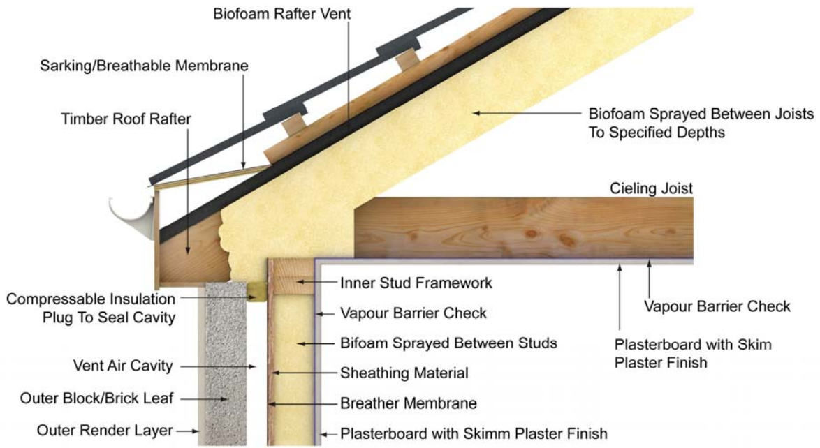
Figure 4: Pitched Roof Construction: non-habitable roof space
