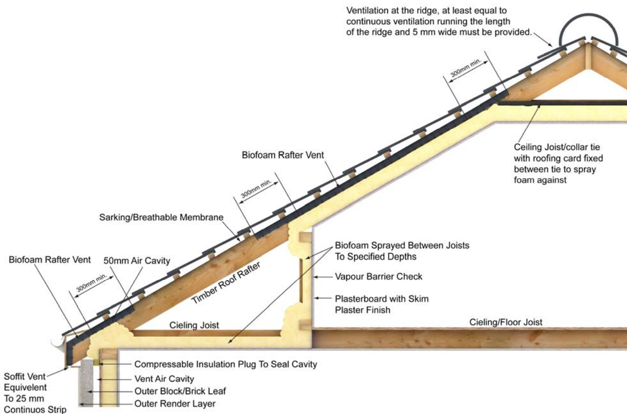
Figure 5: Dormer Roof Construction/Attic Conversion
