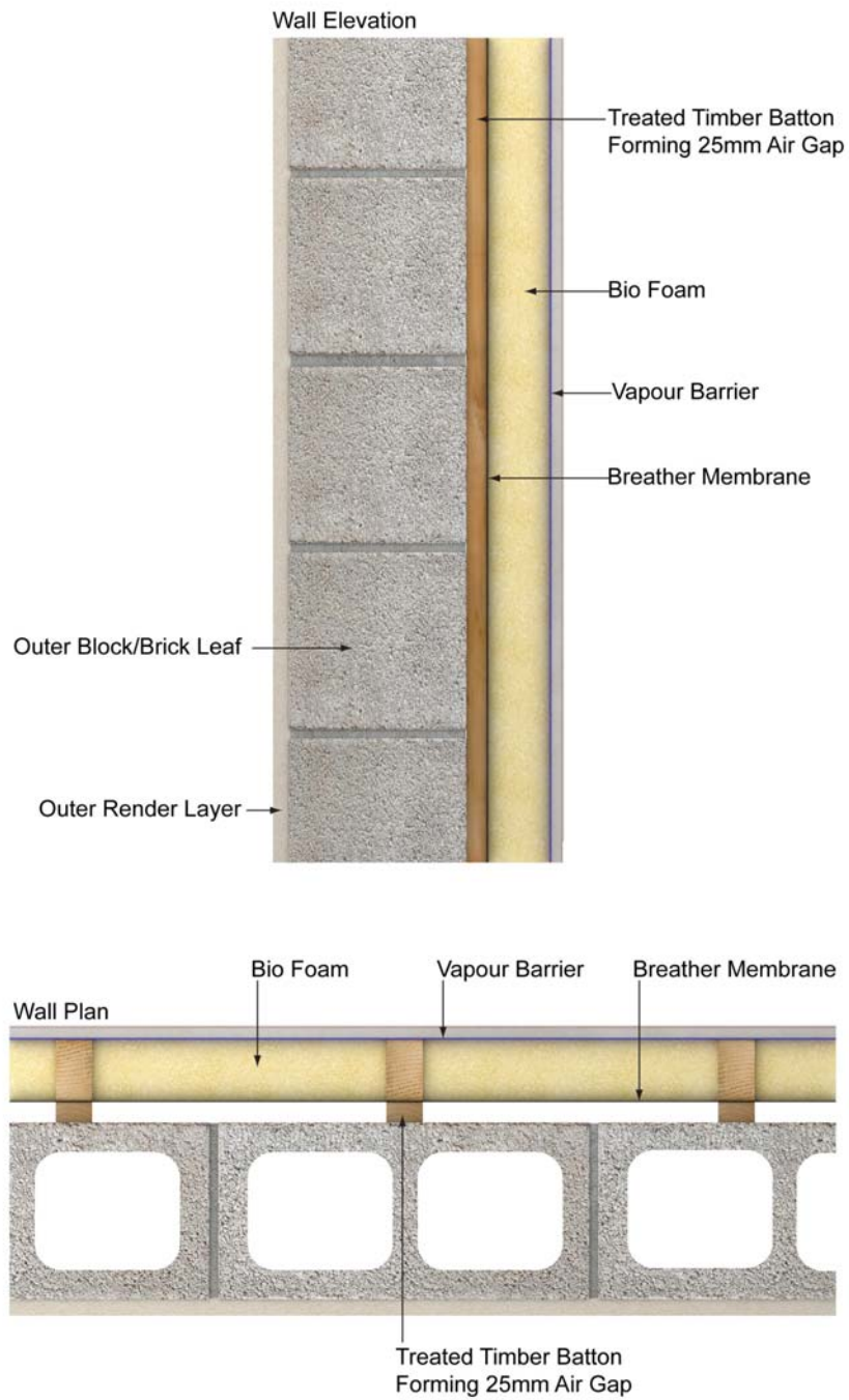
Figure 3: Masonry Wall – Dry Lining
