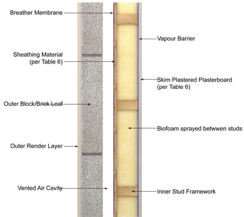
Figure 2: Timber Frame Wall
